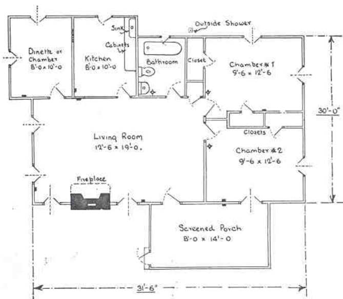
Large Log Cabin, with 2 bedrooms, large living room, separate dinette kitchen, bathroom with tub, outside shower, and screened porch.
