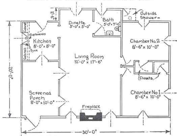
Small model Log Cabin — with 2 Bedrooms, Living Room, Kitchen, Dinette, Bathroom with outside shower and screened porch.
